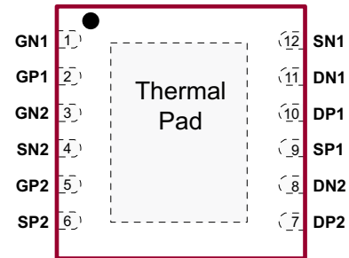
12-Lead DFN (top view)
